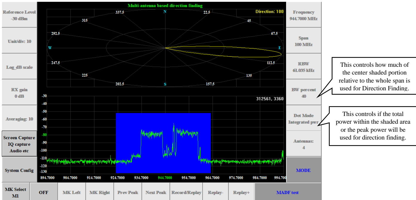
Figure 23, MADF (Multi-Antenna-Direction-Finding) test result example. This shows a simpler 4-antenna system, and the signal direction shows up on the upper polar graph as coming from 100 deg from the North (slightly passing the East direction at 90 deg).
