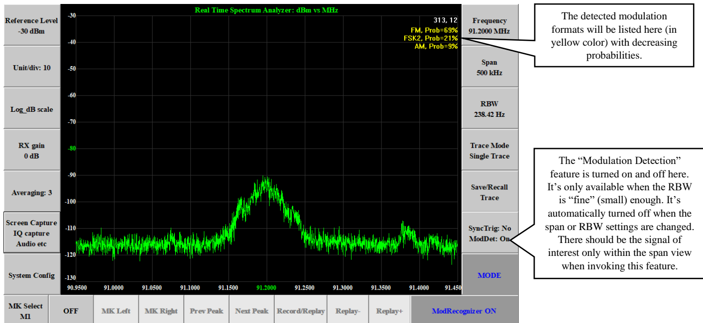
Figure 24, test result example for the Legacy Signal Modulation Detection feature.
